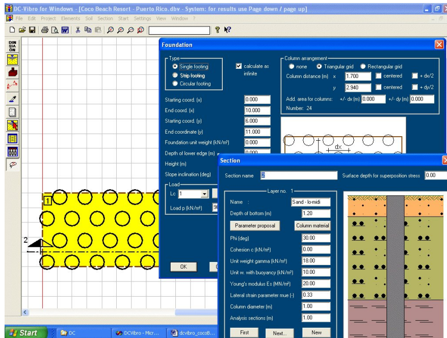
(Figure 3. Program DC-Vibro)
