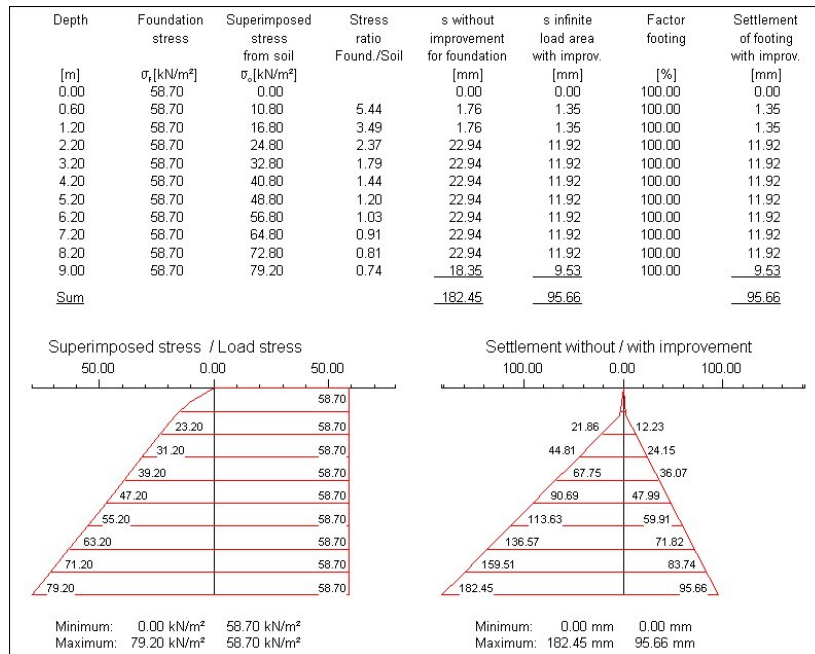
(Figure 4. Settlement analysis and display)
