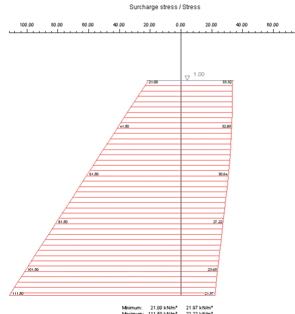
Stresses at the point of evaluation
