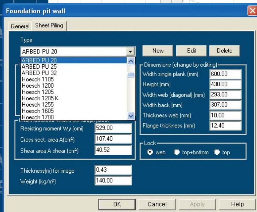
Selection of sheet pile profiles
