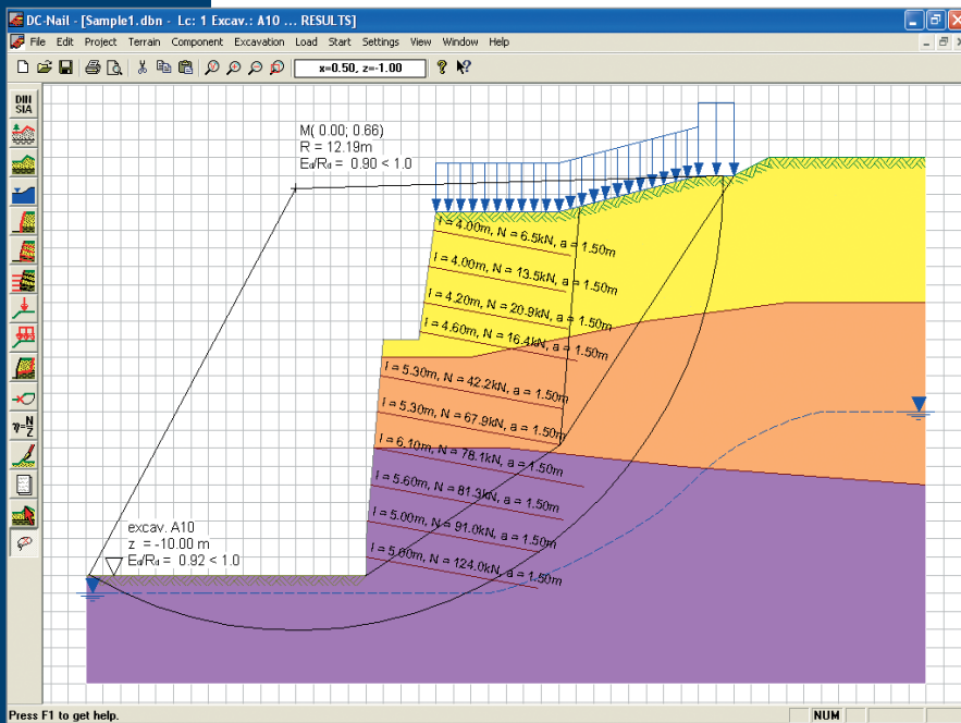
Nail forces and slope stability analysis
