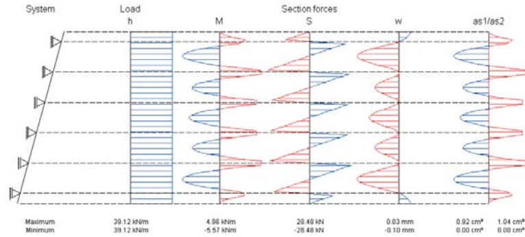
Section forces and reinforcement
